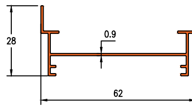
Die No. 19729 0.325KG/M
